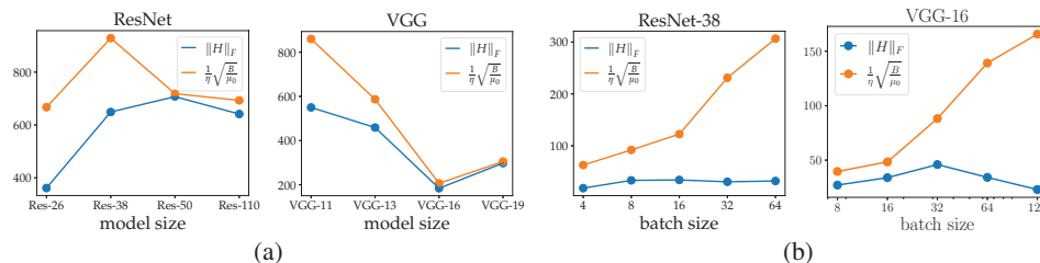
Figure 6: (a) The flatness and upper bound for various ResNets and VGG nets. (b) How the tightness of upper bound changes with decreasing batch size.
