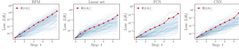
Figure 4: The exponentially fast escape from sharp minima. The blue curves are 200 trajectories of SGD; the red curve corresponds to the average. The sharp minimum is found by GD. When GD nearly converge, we switch to SGD with the same learning rate. This choice ensures that the minimum is stable for GD, and thus the escape is purely driven by SGD noise. For more experimental details, we refer to Appendix A.
