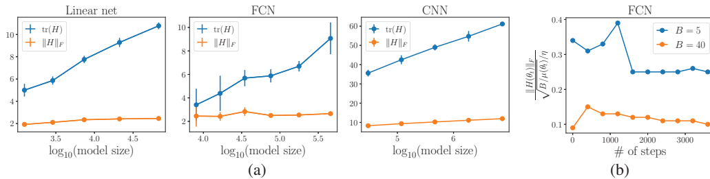
Figure 3: (a) The Frobenius norm and trace of Hessian vs. model size. The error bar corresponds to the standard deviation estimated over 5 runs. (b) The ratio between the Frobenius norm and our upper bound in the training process. Here B = 5 and B = 40 are examined. For more experiment details, we refer to Appendix A.
