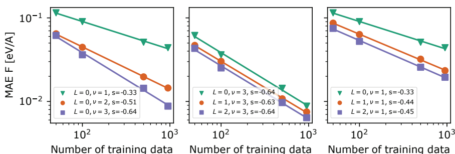
Figure 2: Learning curve of force errors (MAE in eV / Å) for aspirin from the rMD17 dataset for different models. Left : Two layers of invariant ( L = 0 ) MACE with increasing body order \nu \in \{1, 2, 3\} . Center : Two layers of MACE with \nu = 3 and increasing equivariance L \in \{0, 1, 2\} . Right : Two layers of MACE with \nu = 1 and increasing equivariance L \in \{0, 1, 2\} . In each case the slope ( s ) is indicated.
