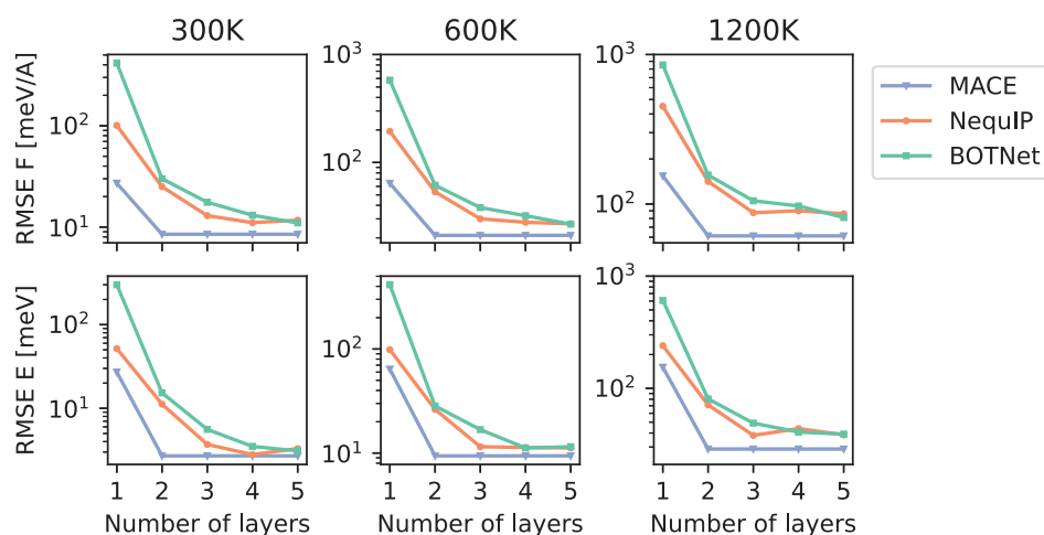
Figure 1: Energy and force errors of BOTNet, NequIP, and MACE ( L = 2 ) on the 3BPA dataset at different temperatures as a function of the number of layers.
