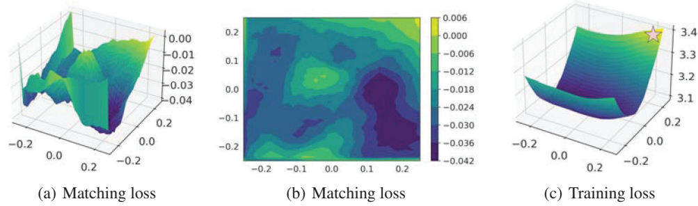
Figure 2: (a) Matching loss defined as 1 - \cos(\nabla \mathcal{L}(x_t, y_{adv}, \theta), \nabla \mathcal{L}(x_i + \delta, y_i, \theta)) , as we vary the perturbation \delta_i projected along two randomly chosen directions. (b) Contour view of (a). (c) Training loss of a single example x_i + \delta_i as we vary \delta_i , projected along two randomly chosen directions. Adding \delta_i^* which minimizes the matching loss to x_i (located at origin), introduces a local region of high training loss (indicated by a star at x_i + \delta_i^* ).
