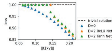
Figure 3: Training loss of D = 2 neural networks with ReLU and Tanh activations across synthetic tasks with different \|\mathbb{E}[xy]\| . We see that with the Kaiming initialization, both the Tanh net and the ReLU net are stuck at the trivial solution in expectation of our theory. In contrast, an optimized linear regressor ( D = 0 ) is better than the trivial solution when \|\mathbb{E}[xy]\| > 0 . See Section A for experimental details.
