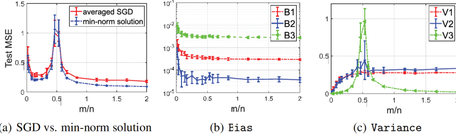
Figure 2: Test MSE (mean±std.) of RF regression as a function of the ratio m/n on MNIST data set (digit 3 vs. 7) across the Gaussian kernel, for d = 784 and n = 600 in (a). The interpolation threshold occurs at m/n = 0.5 as the Gaussian kernel outputs the 2m -feature mapping (instead of m ), i.e., \sigma(\mathbf{W}\mathbf{x}) \in \mathbb{R}^{2m} . Under this setting, the trends of Bias and Variance are empirically given in (b) and (c).
