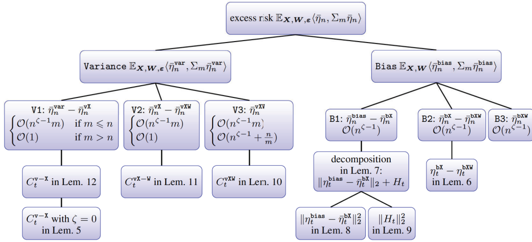
Figure 1: The roadmap of proofs.
