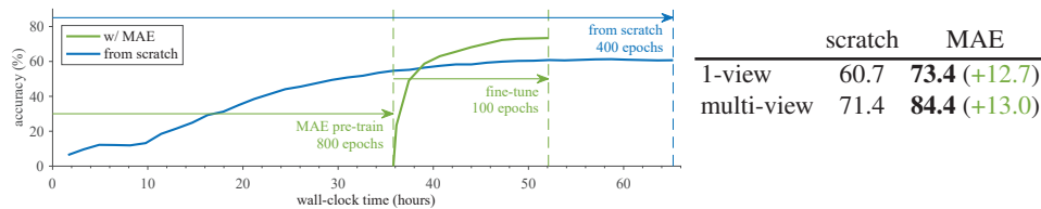
Figure 5: MAE pre-training plus fine-tuning is much more accurate and faster than training from scratch. Here the x-axis is the wall-clock training time (128 A100 GPUs), and the y-axis is the 1-view accuracy on Kinetics-400 validation. The table shows the final accuracy. The model is ViT-L.
