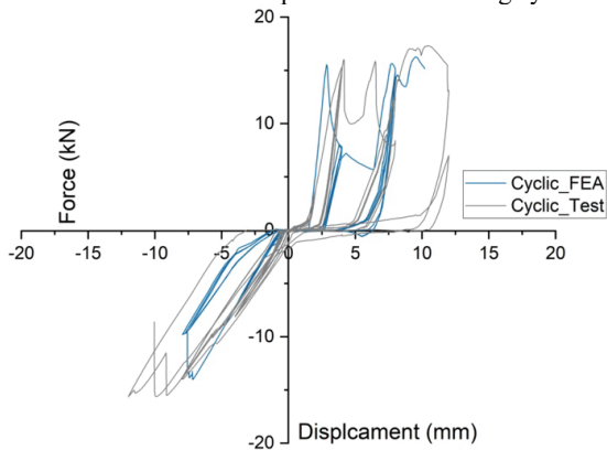
Figure 12: Force-displacement curve of the shear connection [8]
