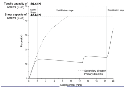
Figure 14: Force and displacement curve of shear connection with S235 and connection deformation on primary (bottom left) and secondary directions (bottom right) under 15mm displacement [8]
