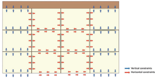
Figure 5: Continuous reinforcement along CLT modules edges provided by assembled connections [8]
