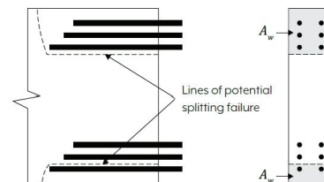
Figure 10: Wood area for checking wood fracture capacity in a knee joint. [26]
