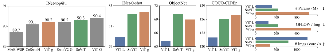
Figure 2: Optimizing for the compute-equivalent of ViT-g/14 results in the 2.5\times smaller SoViT-400m/14 model achieves equivalent results across a wide range of benchmarks. Our model performs exceptionally well on the competitive ImageNet (ILSRV2012) benchmark in comparison with significantly larger models from the recent literature [61, 78, 49, 80].
