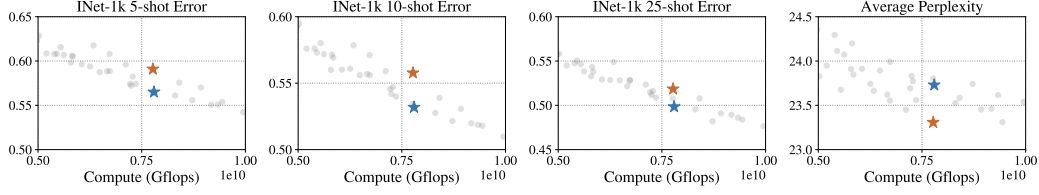
Figure 3: A grid sweep over multiple ViT shapes pretrained on 600M JFT examples highlights the important role of shape. Each dot corresponds to a model architecture pretrained on 600M examples and evaluated on a downstream metric, e.g. Imagenet-1k 5-shot in the leftmost plot. The two architectures marked in blue and red – identical in all four figures – are compute-optimal for classification and image-to-text tasks (captioning/VQA), respectively. For captioning/VQA, we average log-perplexity scores (see Section 4.2). In the leftmost three figures, using Imagenet-1k few-shot evaluation, the compute-optimal model highlighted in blue is compute-optimal in all three cases, but it is not compute-optimal for image-to-text tasks as shown in the rightmost figure. So, in small models, an optimal shape in one domain is not necessarily optimal in others.
