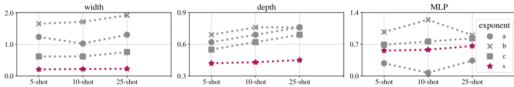
Figure 5: A plot of the estimated values of the exponents in (2) for different evaluation metrics f . The scaling exponent s_k tends to be less sensitive to the choice of metric than other exponents. Moreover, the data scaling exponent c is approximately c \approx 0.65 \pm .06 , independently of the choice of the shape dimension, in agreement with what would be expected using space partitioning arguments [2, 38, 59].
