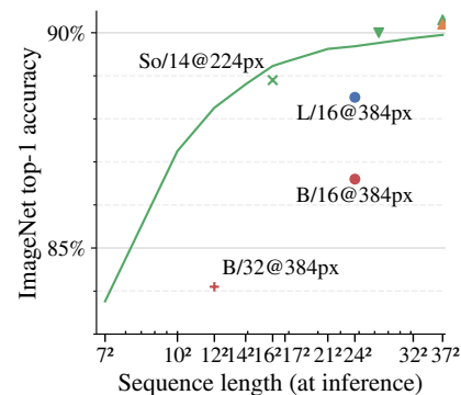
Figure 7: Flexification of SoViT-400m/14 (abbr. So/14). See Section 5.5.
