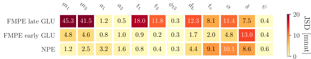
Figure 12: Jensen-Shannon divergence between inferred posteriors and the reference posteriors for GW150914 [73]. We compare two FMPE models with the same architecture as the NPE embedding network, see Tab. 3 bottom panel. For the model in the first row, the GLU conditioning of (\theta, t) is only applied before the final 128-dim blocks. The model in the middle row is given the context after the very first 2048 block.
