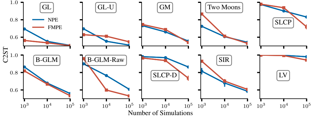
Figure 4: Comparison of FMPE with NPE, a standard SBI method, across 10 benchmark tasks [46].
