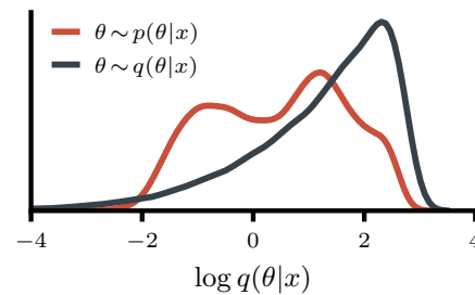
Figure 3: Histogram of FMPE densities \log q(\theta|x) for reference samples \theta \sim p(\theta|x) (Two Moons task, N = 10^3 ). The estimate q(\theta|x) clearly covers p(\theta|x) entirely.
