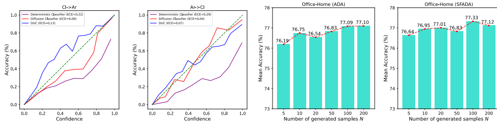
Figure 2: (a) Visualization of Expected Calibration Error (ECE) for ADA on task Ar → Cl and Cl → Ar. (b) Performance under different choices of N on Office-Home for ADA and SFADA.
