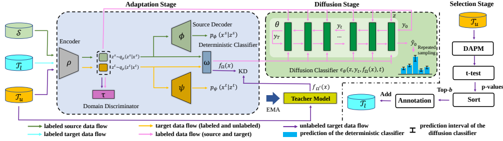
Figure 1: Framework of DAPM. Each active learning round goes through three stages: two stages for training and one stage for selection. Parameters in blue and green backgrounds are trained in the adaptation stage and the diffusion stage, respectively. When the adaptation stage ends, the parameters involved will be frozen. The teacher model f_{\Omega'} is updated by EMA from the student model f_\Omega .
