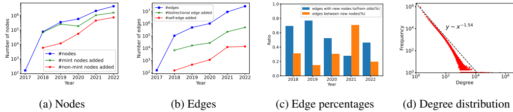
Figure 1: Evolution of nodes and edges.
