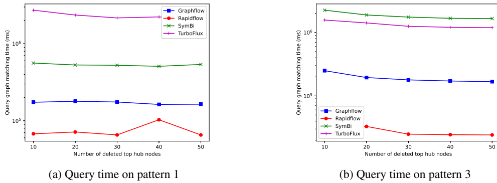
Figure 9: Query time with deleted hub nodes.
