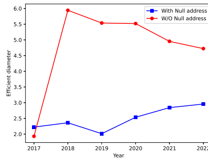
Figure 8: Effective diameter by years.
