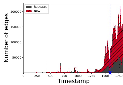
(a) TEA plot with day intervals
