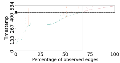
(b) TET plot with sampled 2 million edges
