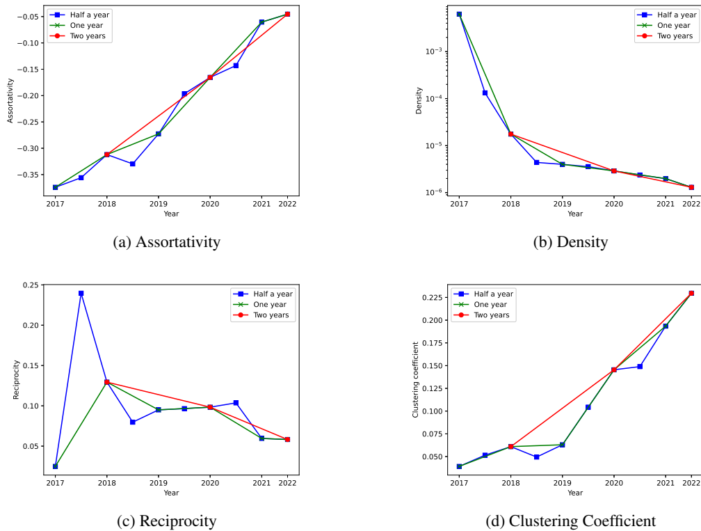
Figure 4: Evolution of network global properties with different time granularity.
