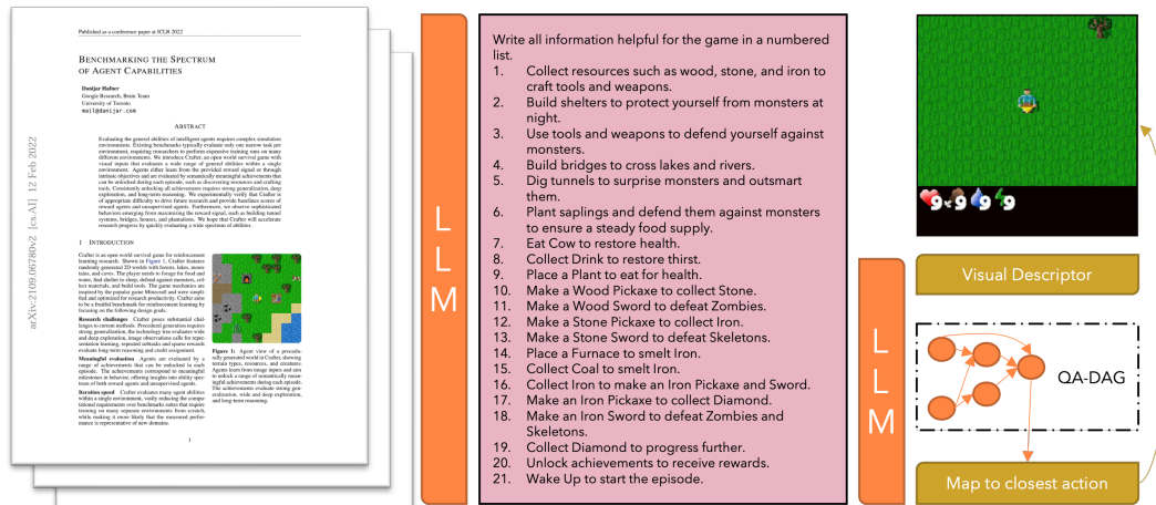
Figure 1: Overview of SPRING. The context string, shown in the middle column, is obtained by parsing the \text{\LaTeX} source code of Hafner (2021). The LLM-based agent then takes input from a visual game descriptor and the context string. The agent uses questions composed into a DAG for chain-of-thought reasoning, and the last node of the DAG is parsed into action.
