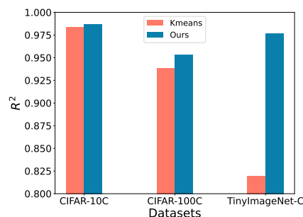
Figure 6: Compare with K-means.
