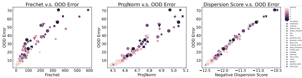
Figure 3: OOD error prediction versus True OOD error on CIFAR-10 with ResNet50. We compare the performance of Dispersion Score with that of ProjNorm and Fréchet via scatter plots. Each point represents one dataset under certain corruption and certain severity, where different shapes represent different types of corruption, and darker color represents the higher severity level.
