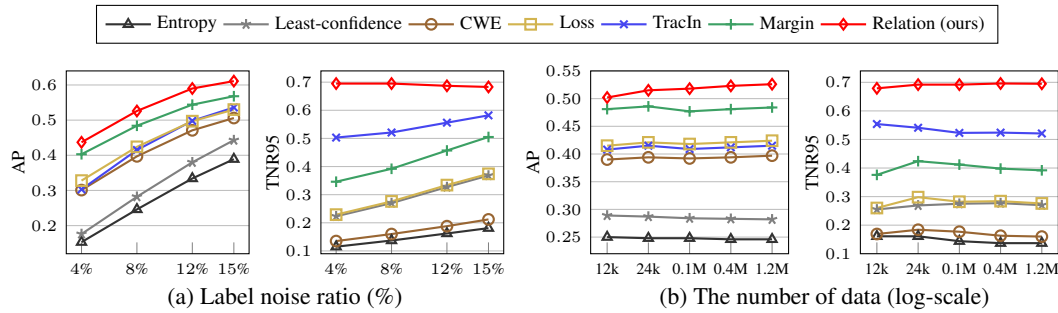
Figure 5: Label error detection performance on ImageNet with MAE-Large according to (a) label noise ratios and (b) the number of data. We obtain the results in (b) with 8% label noise. We report performance values of all methods in Appendix D.3, with Tables 10 and 11.
