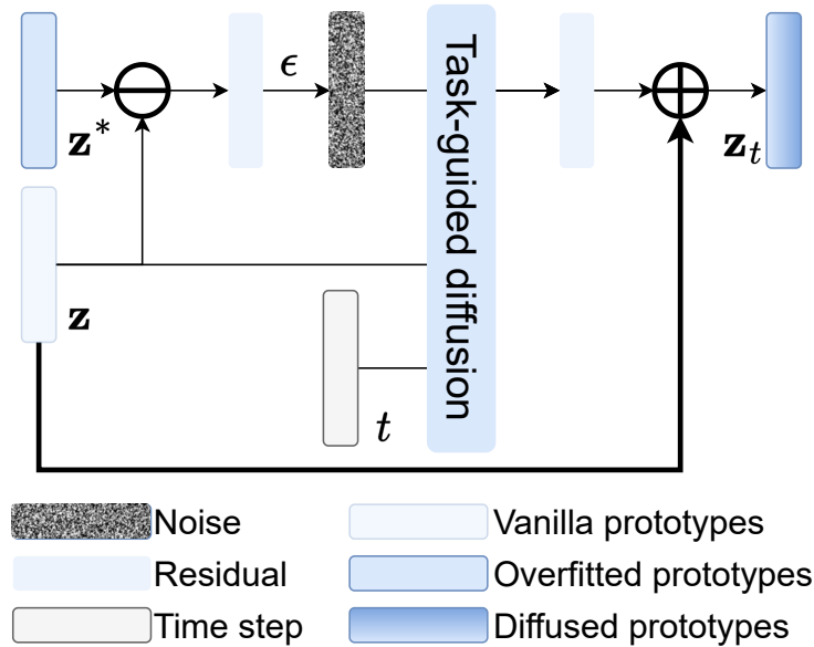
Figure 9: Residual prototype learning.
