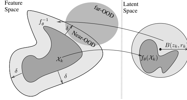
Figure 1: Illustration of the representation mapping in Theorem 1 with the conditions to detect far OOD nodes (Theorem 6) and near OOD nodes (Corollary 7).
