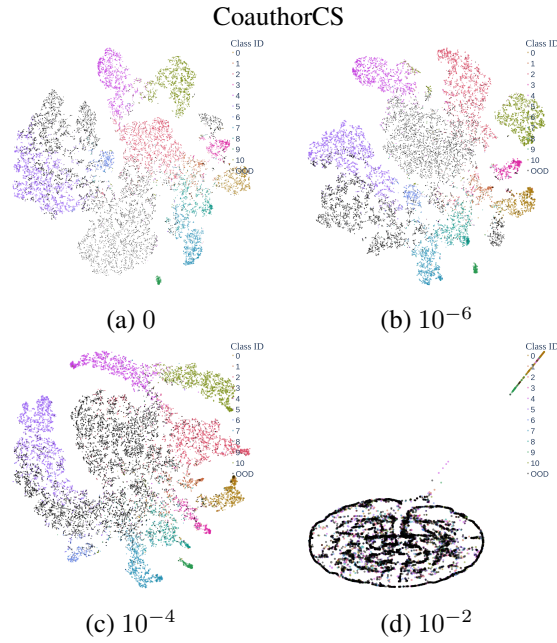
Figure 4: latent representation for Coauthor CS
