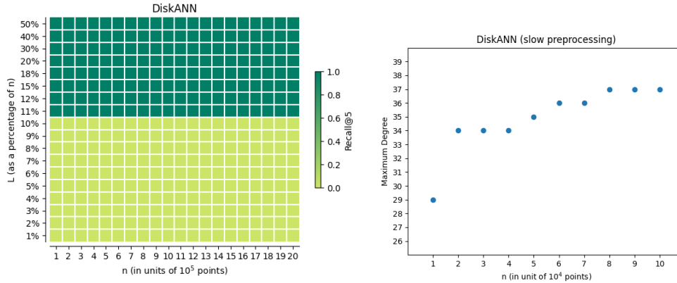
Figure 3: Results for both variants of the DiskANN algorithm on the instance in Figure 2. Left figure (fast preprocessing DiskANN): the horizontal axis represents the data size n , in multiples of 10^5 points. The vertical axis represents the size of the search queue length L in terms of the percentage of the data size. Each pixel represents the average value of Recall@5 \in [0, 1] over 10 runs of the algorithm. Note the sharp transition of the recall (from 0 to 1) for L \approx 10\% . Right figure (slow preprocessing DiskANN): as indicated by Theorem 3.4, slow preprocessing DiskANN constructs a very efficient data structure. In the experiment, it finds the exact nearest neighbor in at most 2 steps of greedy search, with L = 1 . In the figure we plot the maximum degree of the constructed graph (on the vertical axis) vs. the data size n in multiples of 10^4 points (on the horizontal axis). The plot ends at n = 10^5 , as the slow preprocessing algorithm takes several hundred hours for larger values of n .
