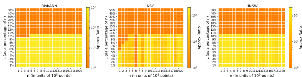
Figure 6: Average approximation ratio results for running DiskANN (fast preprocessing), NSG, and HNSW algorithm on instances in Figure 2 and 4. The horizontal axis depicts the data size n , in multiples of 10^5 . The vertical axis depicts the size L of the search queue, as a ratio to n . Each pixel represents the average approximation ratio over 10 runs of the algorithm. Since the algorithms are randomized, each run generates and uses a different random seed.
