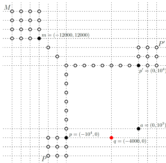
Figure 4: Our constructed hard instance for NSG and HNSW algorithms for data size n = 10^6 . The instance lives in a two-dimensional Euclidean space, and therefore has a constant doubling dimension. Black dots (solid or hollow) are points in the database, the red dot is the query point. Grids are only used to show the layout structure. See Section 4.2 for a detailed description and supplementary materials for its implementation.
