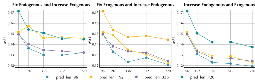
Figure 3: Performance with the enlarged look-back length varying from {96, 192, 336, 512, 720}. Different styles of lines represent different prediction lengths. In most cases, the forecasting performance benefits from enlarged look-back lengths of both endogenous and exogenous series.
