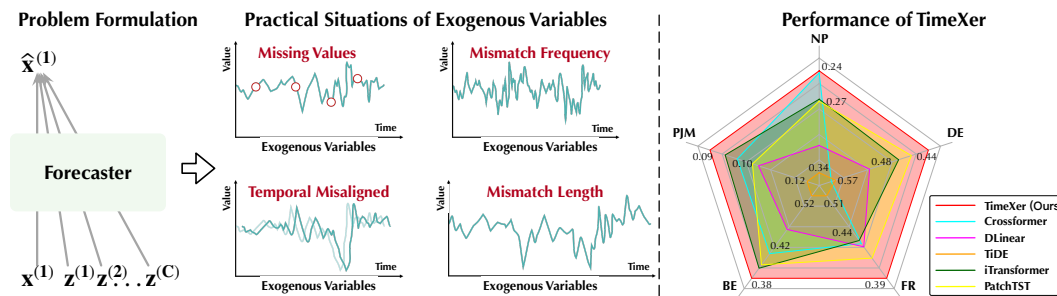
Figure 1: Left: The forecasting with exogenous variables paradigm includes inputs from multiple external variables as auxiliary information without the need for forecasting. Right: Model performance comparison on existing electricity price forecasting with exogenous variables benchmarks.
