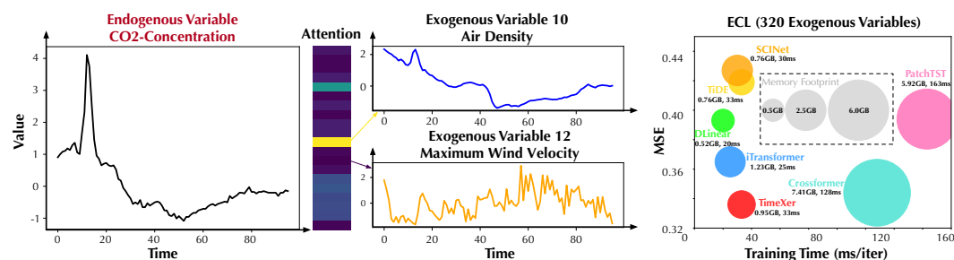
Figure 5: Model analysis of TimeXer. Left: Visualization of learned attention map and the endogenous time series and exogenous time series with highest and lowest attention scores. Right: Model efficiency comparison under the forecasting with exogenous variables paradigm on the ECL dataset.
