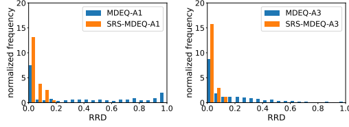
Figure 2: RRD histogram with MDEQ-LARGE with 20 bins.
