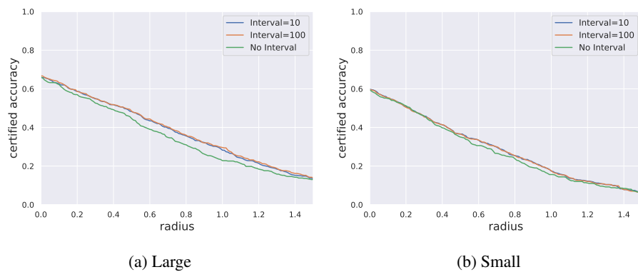
Figure 12: Different warm-up restart intervals for SRS-MDEQ-3A.
