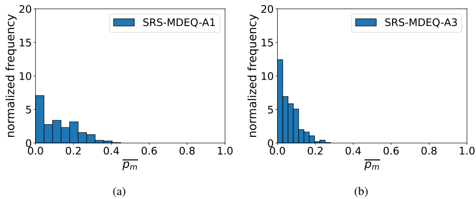
Figure 7: \overline{p}_m histogram with MDEQ-SMALL models. There are 10 bins in each histogram.
