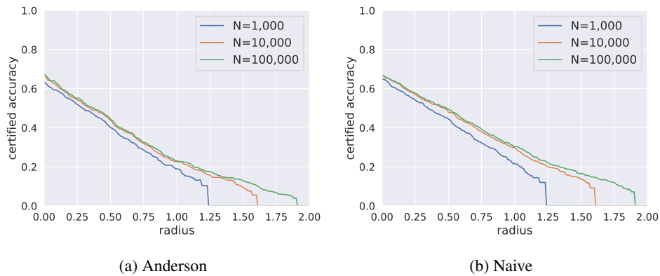
Figure 9: Different number of samplings for MDEQ-LARGE with the 3-step solvers.
