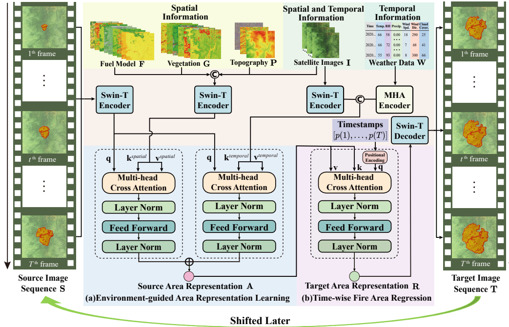
Figure 3: S2R-FireTr forecasts wildfires by predicting future target fire areas based on source fire areas. (a) During the environment-guided area representation learning, we input the source fire areas and multi-modal environmental information into the transformer to compute the source area presentation A . (b) During the time-wise fire area regression, we input the source area presentation A and the target timestamp into the transformer to compute the target area presentation R for predicting the target fire areas. “ Shifted Later ” means that we concatenate the source and target areas to predict later areas. Source and target areas can be interchanged, creating a pipeline for wildfire backtracking.
