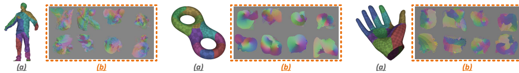
Figure 11: Results of Nuvo: (a) input meshes (different colors denote chart assignment); (b) chart-wise UV maps.
