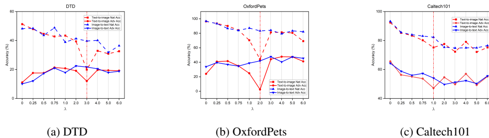
Figure 4: Instability analysis for DTD, OxfordPets, and Caltech101. We report the model performance (%) w.r.t the ratio ( \lambda ) between natural and robust terms in training objectives. The results of deep prompt interaction from text to image are plotted in red line, while that from image to text are plotted in blue line.
