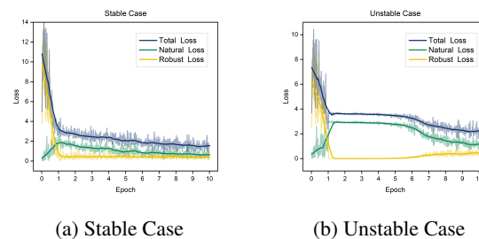
Figure 5: Training loss curve under both stable and unstable settings. We report the total, natural, and robust loss during the whole training stage.
