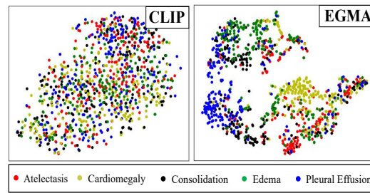
Figure 4: t-SNE visualization on CheXpert 5x200 dataset by CLIP and our EGMA. The figures display points of different colors representing various ground truth disease types and their cluster assignments. The color-coded points illustrate the clustering results of each algorithm.
