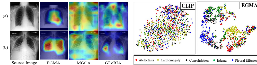
Figure 3: Results of cross-modality attention maps visualization. Related text content: (a) "heart size borderline enlarged"; (b) "increased bibasilar opacities are the combination of increased bilateral pleural effusions and bibasilar atelectasis".
