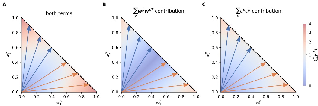
Figure A.8: Specialized students and gates accelerate adaptation. Heatmaps of the dot product (\frac{d}{dt} \mathbf{y})^T \varepsilon contributions for different terms of the Neural Tangent Kernel (NTK), depending on specialization of weight vectors \mathbf{w}^1 (blue), \mathbf{w}^2 (orange), of which three pairs corresponding to different degrees of specialization are shown here (pairs are formed by vectors that are symmetric along the diagonal). c^1, c^2 are scaled so that the sum lies on the dashed black line (given by L^1 regularization). A. shows the total contribution of both terms of Eq. (20) combined, B. isolates the contribution from the \mathbf{w}^p \mathbf{w}^{pT} term, and C. displays the contribution from the c^p c^p term. Dashed lines indicate possible solutions.
