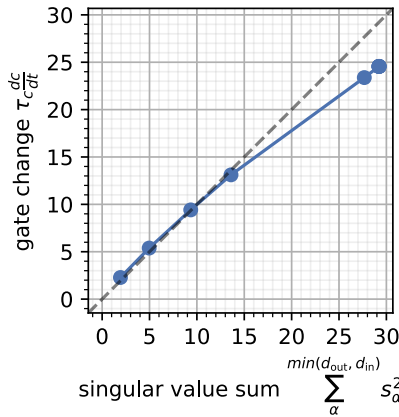
Figure A.2: High-dimensional students learn slower. Gate change \tau_c \frac{dc}{dt} as a function of teacher dimensionality/rank (i.e., non-zero singular values). Weight scaling is chosen such that input and output components take unit scale, y_i = \mathcal{O}(1) , x_j = \mathcal{O}(1) .
