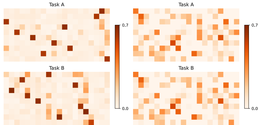
Figure A.5: Regularized, but not non-regularized, fully-connected network specializes single neurons in each row as ‘gates’ per task and exhibits specificity based on task. Visualization of the unsorted second hidden layer of the flexible ( left ) and forgetful ( right ) fully-connected network for a single seed.
