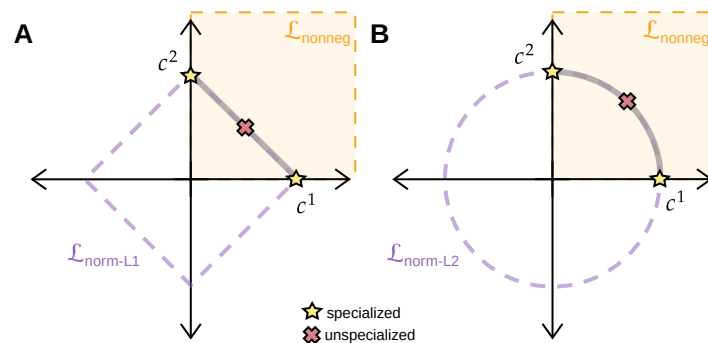
Figure B.1: The effect of regularization on gating variables. Regularization encourages competition between gates while preventing degeneracy of solutions. Importantly, regularization does not force gating variables to be specialized, as illustrated by the red \times . This holds for two regularizers we consider, A. \mathcal{L}_{\text{norm-L1}} and B. \mathcal{L}_{\text{norm-L2}} .
