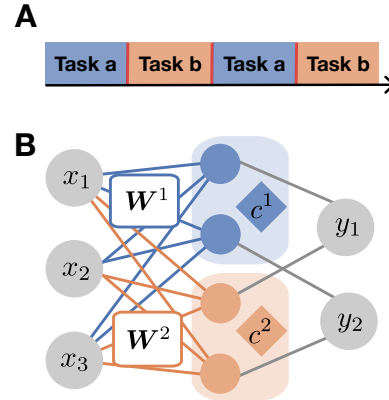
Figure 1: The open-ended learning setting and the modeling approach. A. Example of the blocked curriculum with two tasks. B. Neural Task Abstraction (NTA) model updates W^p through gradient descent, but also the gating variables c^p , leading to task abstractions emerging in the gating layer.
