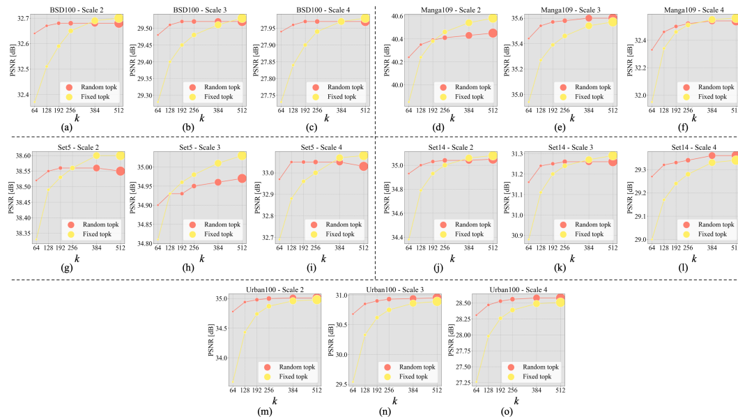
Figure 12: Ablation study on the impact of k for Image SR with SemanIR-B on BSD100 (a-c), Manga109 (d-f), Set5 (g-i), Set14 (j-l) and Urban100 (m-o) datasets with scale = (2\times, 3\times, \text{ and } 4\times) .
