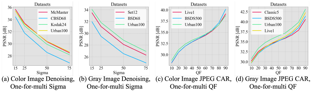
Figure 5: One model is trained to handle multi-degradations for denoising (a-b) and JPEG CAR (c-d).
