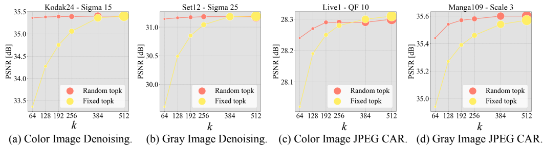
Figure 3: The impact of k with different inference k value. Circle size represents FLOPs.
