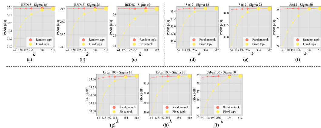
Figure 11: Ablation study on the impact of k for Grayscale Image Denoising on BSD68 (a-c), Set12 (d-f), and Urban100 (g-i) datasets with \sigma = \{15, 25, 50\} .
