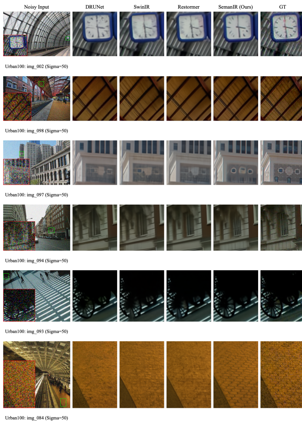
Figure 17: Visual comparison with image denoising on Urban100 dataset. Best viewed by zooming.
