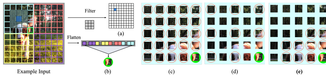
Figure 1: (a) The CNN filter captures information only within a local region. (b) The standard MLP/Transformer architectures take full input in a long-sequence manner. (c) The window-size multi-head self-attention (MSA) mechanism builds a full connection within each window. (d) Position-fixed sparse connection. (e) The proposed Key-Semantic connection.
