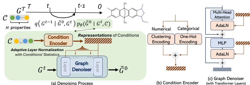
Figure 2: Denoising framework and architectures for Graph DiT. Details are in Section 3.2.
