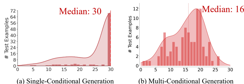
Figure 6: We compare the average ranking of generated polymers with desirable properties. First, we generate three sets of polymers using a single-conditional approach for each condition. In (a), as shown in Figure 1, we find the ranking of the shared structure for each multi-condition requirement. In (b), polymers are generated using a multi-conditional approach, and for each, we identify the highest ranking among the three single-conditional sets. Then, we calculate the median of these maximum ranking positions, which is 16, approximately 2\times better than single-conditional generation, which has a median value greater than 30.
