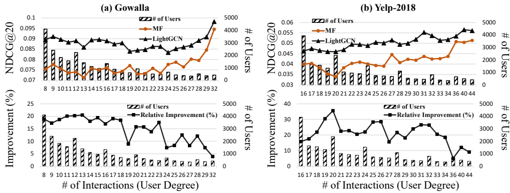
Figure 1: Performances of LightGCN and Matrix Factorization w.r.t. the user degree across datasets. The performance improvement brought by message passing decreases as the user degree goes up.
