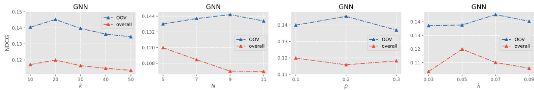
Figure 6: Hyperparameter analysis of GNN backbone on CiteULike dataset
