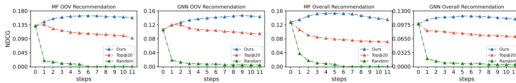
Figure 4: Performance analysis of different generation methods on the CiteULike dataset.
