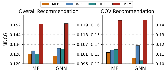
Figure 3: Comparing USIM with other RL methods for overall and OOV recommendation performance in CiteULike dataset.
