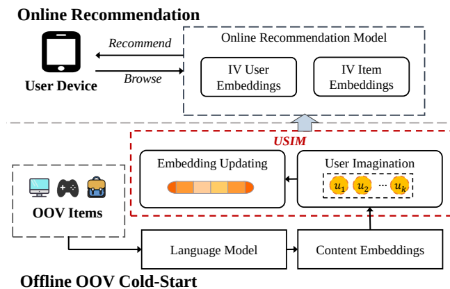
Figure 7: Overall framework of online implementation.
