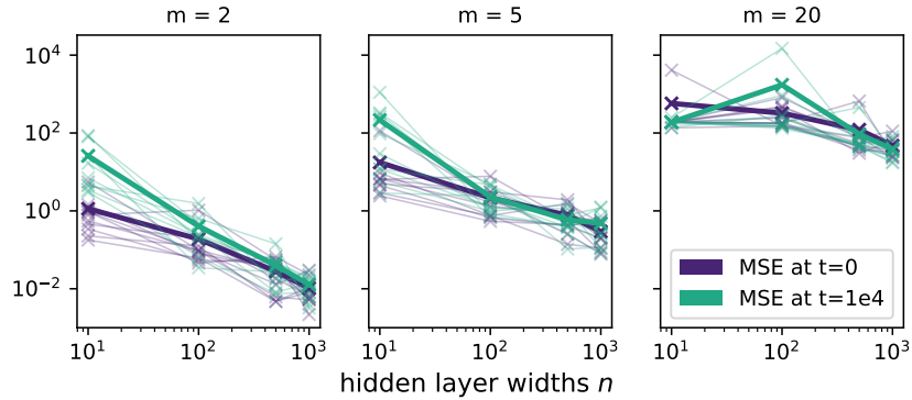
Figure B.3: Mean squared errors between empirical NTKs and analytic NTKs in Figure 1 for all 10 networks (thin lines) and averaged over the 10 networks (thick lines).
