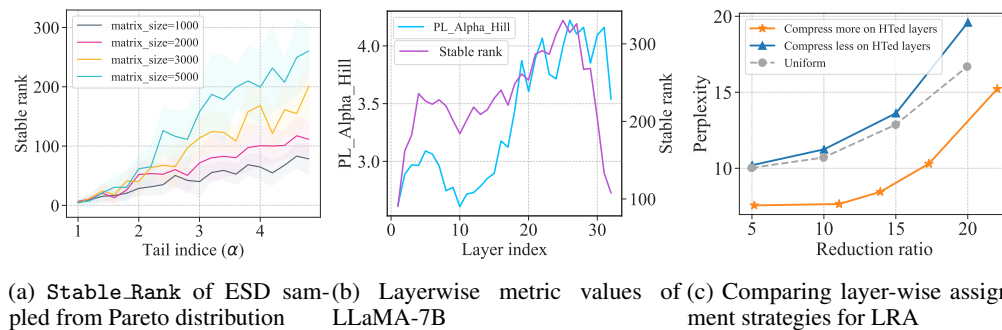
Figure 9: Analyzing ESD properties and assignment strategies for LRA. (a) Stable_Rank and PL_Alpha_Hill show a similar pattern (the more heavy-tailed, the more low-ranked) across different ESDs sampled from Pareto distribution. (b) The layer-wise PL_Alpha_Hill and Stable_Rank of the LLaMA-7B model exhibit a similar trend. (c) Comparing two assignment strategies for LRA, and “Compress more on HTed layers” is better. This finding is opposite to pruning-based methods, which find that “Compress less on HTed layers” is better.
