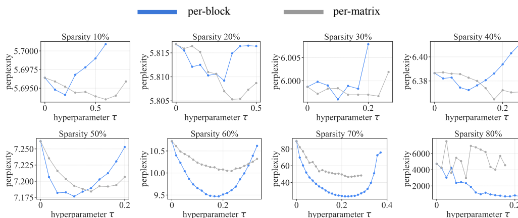
Figure 12: Ablation study on sparsity allocation function hyperparameter \tau . We use Wanda to prune LLaMA model using AlphaPruning with both per-matrix and per-block allocation methods.
