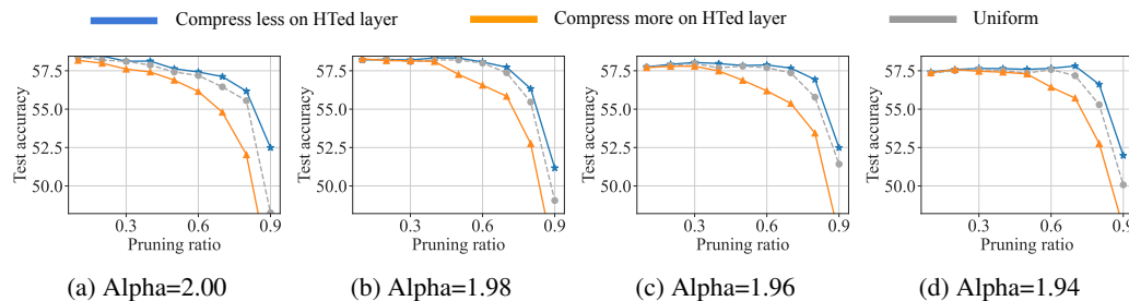
Figure 11: Comparison of our proposed layer-wise assignment strategy with other strategies on models with varying model-wise HT measures. “Compress less on HTed layer” (AlphaPruning) consistently outperforms Uniform pruning across different models, while “Compress more on HTed layer” leads to worse performance compared to Uniform pruning. The experiments used FCNs trained on CIFAR-10.
