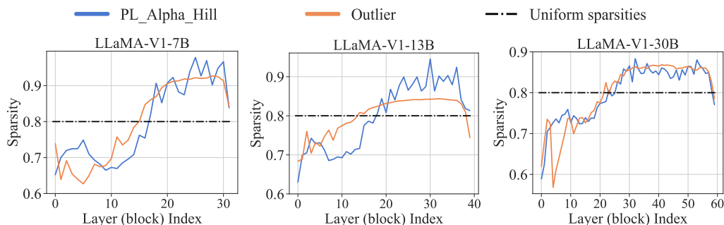
Figure 7: Comparing layer-wise sparsity distributions allocated by AlphaPruning (blue, ours) and OWL (orange). While both methods show similar overall trends, AlphaPruning generates a more granular distribution with distinct differences between consecutive layers.
