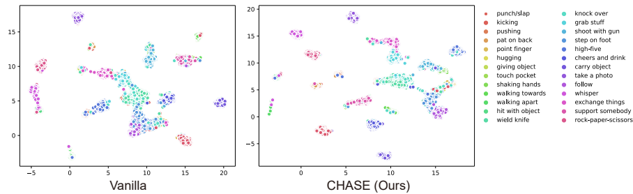
Figure 5: UMAP [100] visualizations of multi-entity skeleton sequence representations on the test split of NTU Mutual 26 X-Sub. Compared with Vanilla, our proposed CHASE differentiate similar multi-entity actions better by assisting backbones to learn more distinctive representations.
