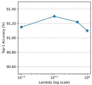
Figure 10: Ablation study on different \lambda s for MPMMD.
