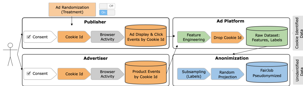
Figure 7: Data collection and processing overview.
