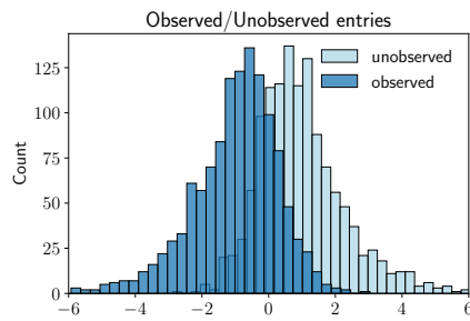
Figure 1: Observation bias with variance \sigma^2 = 1 .
