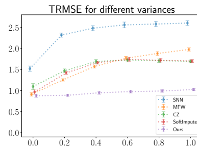
Figure 2: TRMSE with standard error for different variances \sigma^2 = 0.0, 0.2, 0.4, 0.6, 0.8, 1.0 .
