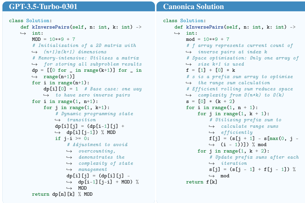
Figure 2: A case illustration of GPT-3.5-turbo-0301 and canonical_solution . GPT-3.5-turbo-0301 generated code requires 70.62x memory usage compared with canonical_solution . GPT-3.5-turbo-0301 generated code employs a 2-dimensional matrix to manage state transitions, leading to substantial memory overhead, particularly evident when the parameters n and k are large. In contrast, the canonical_solution optimizes memory usage by utilizing a rolling sum technique and a single-dimensional dynamic array, significantly reducing the space complexity from O(n \times k) to O(k) .
