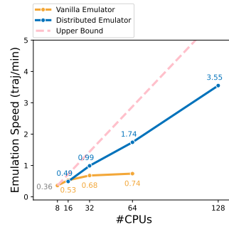
Figure 22: Emulation speed w.r.t number of CPUs used. The upper bound can only achieved when there is no communication and error handling cost. Our design of distributed emulator can significantly improve the efficiency of emulation compared to the vanilla method of running all emulations over the same instance.
