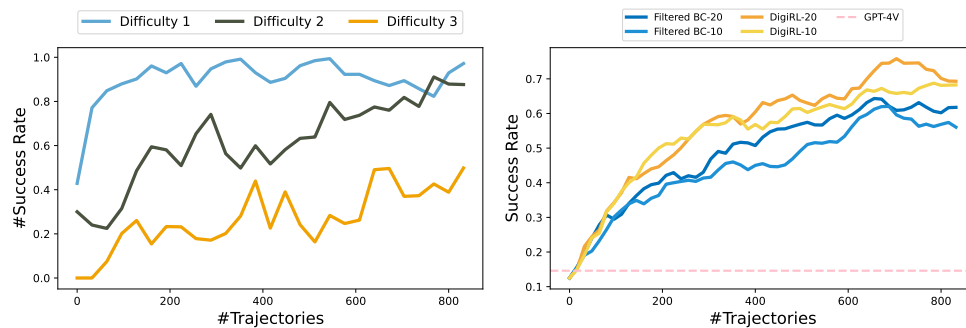
Figure 10: Left: Success rate under different difficulties for the AitW Webshopping task set. Right: Success rate under different methods with different horizon length ( H \in \{10, 20\} ) on the AitW Google Search task set.
