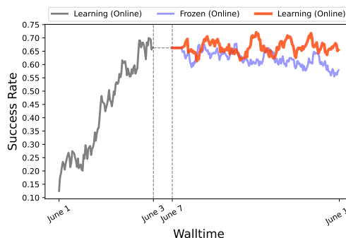
Figure 4: Performance of our approach (DigiRL) in different training modes on the Webshop subset. When utilizing a stale checkpoint, i.e., “frozen” (black+blue curve) performance generally begins to degrade as time evolves, whereas autonomous online training (black+red curve) via DigiRL allows us to retain performance despite non-stationarity and stochasticity.
