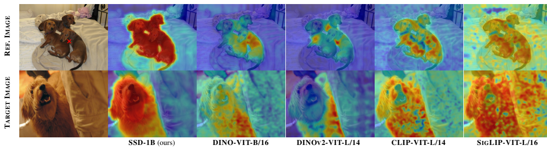
Figure 4: Qualitative results on the semantic coherence of various vision encoders. We select a patch (red marker) associated to the dog in REF. IMAGE. Top row shows the cosine similarity heatmap between the selected patch and all patches produced by vision encoders for REF. IMAGE. Bottom row shows the heatmap between the selected patch in REF. IMAGE and all patches produced by vision encoders for TARGET. IMAGE.
