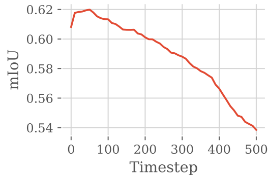
Figure 7: mIoU according to the noising timestep on Pascal VOC.
