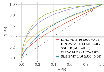
Figure 3: ROC curves revealing the semantic coherence of vision encoders.
