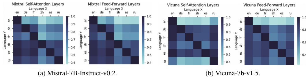
Figure 5: Overlapping ratio of language-specific neurons in self-attention and feed-forward structures.
