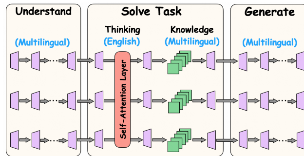
Figure 2: Our hypothesized multilingual workflow, MWork , converts multilingual queries to English for reasoning in English and generates responses in the original language, demonstrating a layered processing approach.
