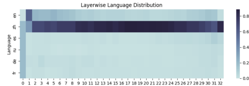
Figure 7: Ratio of languages among layers in Chinese Llama given non-English instructions.
