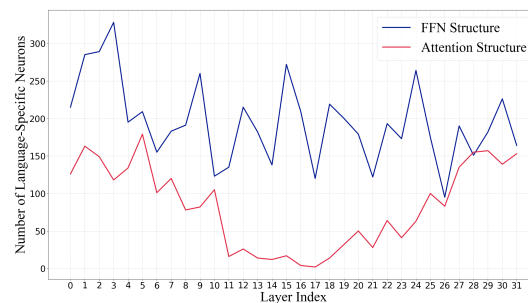
Figure 3: Number of language-specific neurons when processing multilingual queries.
