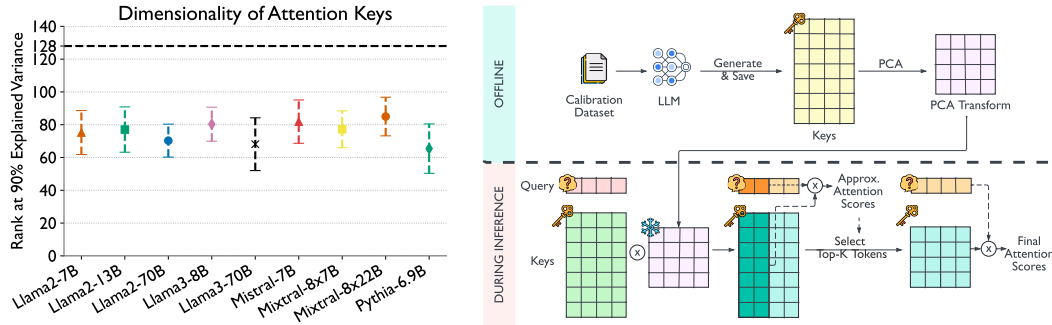
Figure 1: Rank at which 90% of the variance is explained, averaged across all layers and heads for different models. Full rank is represented by the black dashed line (left). Overview of Loki (right).
