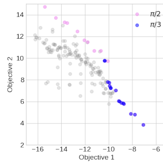
Figure 1: Effect of cone selection on size of Pareto optimal set
