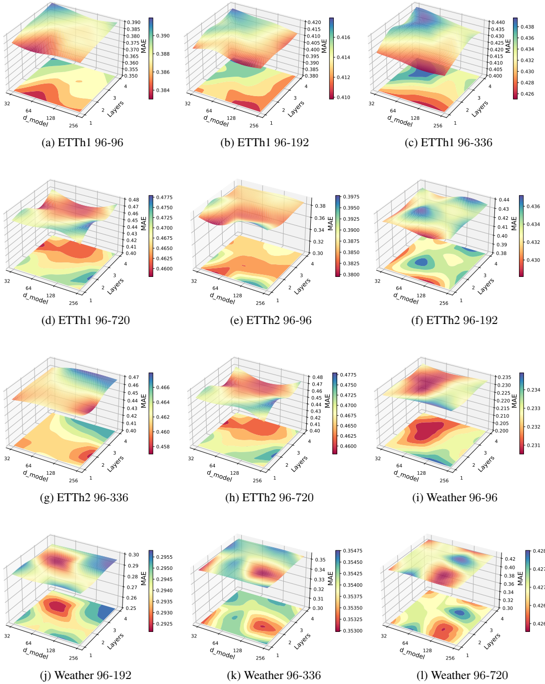
Figure 16: Sensitivity analysis of model capacity-related hyper-parameters d_{model} and number of layers L . Experiments are carried out on typical long-term forecasting datasets, including ETTh1, ETTh2, and Weather datasets. “96-96/192/336/720” denotes different forecasting length settings
