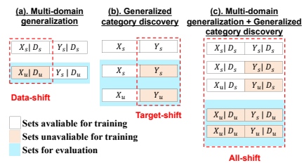
Figure 2: Diagrams of different generalization settings in visual classification tasks.
