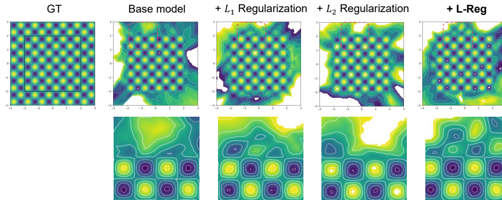
Figure 6: Prediction visualizations of MLP with different regularization terms.
