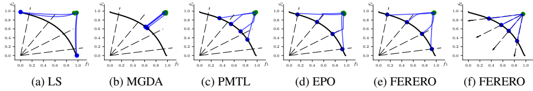
Figure 3: Converging solutions (blue dots) and optimization trajectories (blue lines) on the objective space of different methods on synthetic objectives given in (5.1). Dashed arrows represent pre-specified preference vectors. The green dots represent initial objective values.
