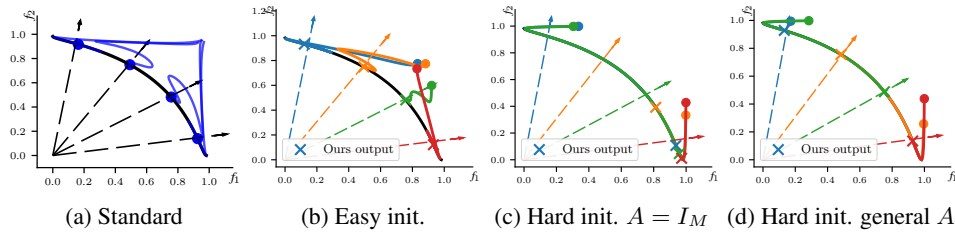
Figure 8: Synthetic experiment results with Algorithm 2.
