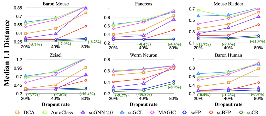
Figure 10: Performance on dropout recovery, measured by L1 Median Distance. Figures highlighted in green indicate reduction rates from the most competitive baseline at each setting.
