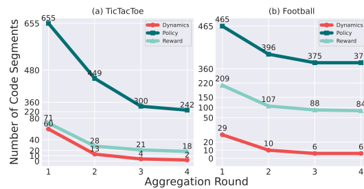
Figure 3: Knowledge Segment Aggregation.
