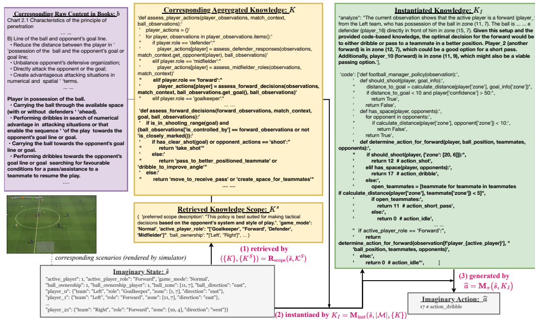
Figure 5: An example of the URI data generation process in the football game. The imaginary state \hat{s} is collected from the real environment, which is 12 timesteps of a football game, while the rendered image is the corresponding scenario generated by the simulator. The imaginary action is "dribble", where the logic is supported by the "has_space" branch in K_I . Based on this, we bold the relevant information in the predecessor nodes and skip irrelevant information with the ellipsis "...".
