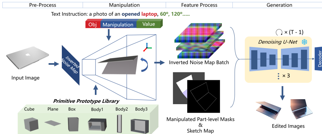
Figure 2: The overall image editing process. (1) In the Pre-Process stage, articulated objects in 2D images are part-level segmented and reconstructed to abstract 3D models. Meanwhile, inverted noise maps of input images are created with DDIM Inversion. (2) In the Manipulation stage, various manipulations can be implemented based on text instructions or human interaction in the 3D space. (3) After manipulation, part-level masks and sketches are rendered and exported. The inverted noise maps are transformed according to these masks. (4) Finally, with the transformed inverted noise maps, sketch maps, and part-level masks, the generation model creates the edited images.
