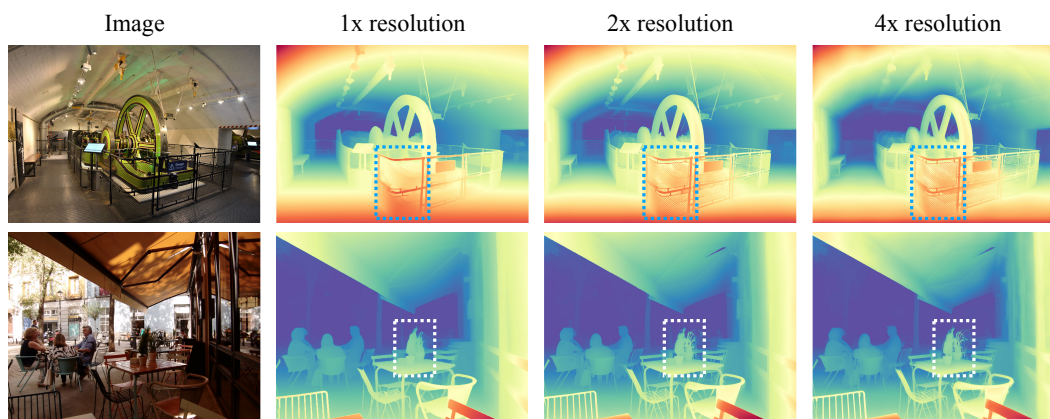
Figure 11: Test-time resolution scaling up can further improve the prediction sharpness.
