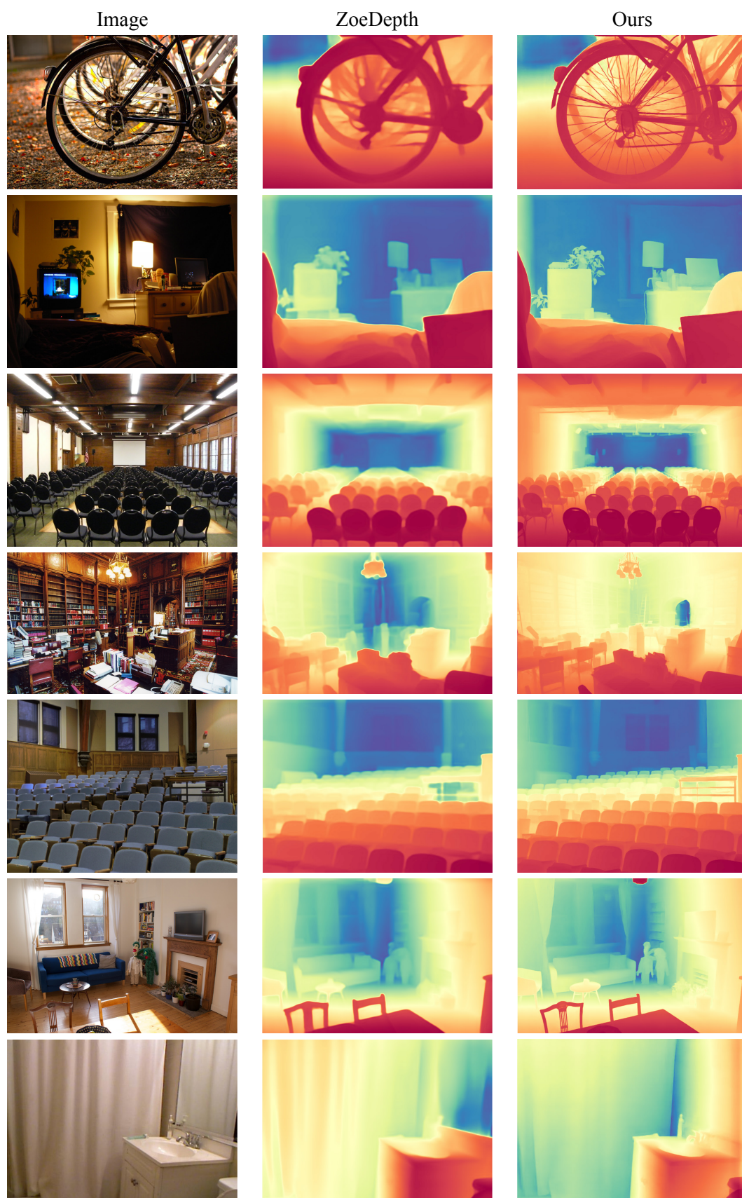
Figure 15: Comparison between ZoeDepth [6] and our fine-tuned metric depth model.
