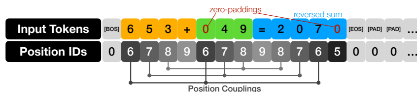
Figure 2: Position coupling for decimal integer addition task, displaying 653 + 49 = 702 with appropriate input formats. The starting position ID ‘6’ is an arbitrarily chosen number.
