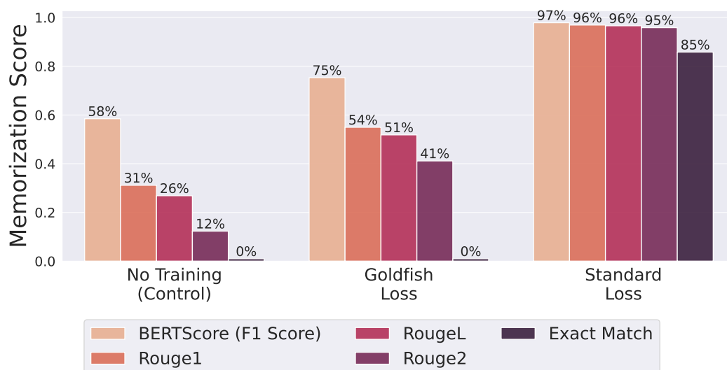
Figure 10: Semantic Memorization: In addition to Rouge1 and Rouge2 measuring unigram overlap and bigram overlap, we also measure BERTScore [Zhang* et al., 2020] which is BERT embedding-based scores where a higher score suggests a closer semantic similarity to the ground truth. Despite the 4-goldfish model’s deterrence to regenerate the exact sequences seen during training, the increased BERT embedding-based BERTScore and n-gram-based Rouge scores (in comparison to Control) suggest that paraphrases might still be leaked. This observation implies that while the model does not memorize, it still learns and retains knowledge from the underlying data.
