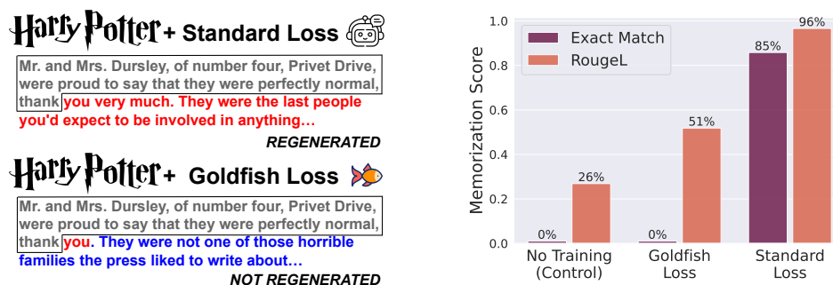
Figure 1: A pretrained 7B model (the control) is further trained for 100 epochs on (left) the first chapter of Harry Potter or (right) 100 wikipedia documents. We observe a drop in exact match memorization and RougeL metrics when training with goldfish loss (see Section 4 for metric descriptions). When prompted with the opening of Harry Potter (gray) the standard model regenerates the original text (red) while the goldfish model does not.
