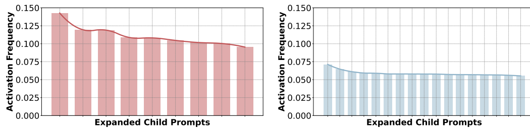
Figure 6: The distribution of logit activation of the learned prompts in the 2nd round ( left ) and the 3rd round ( right ). The prompt of the highest activation frequency is identified for further expansion.
