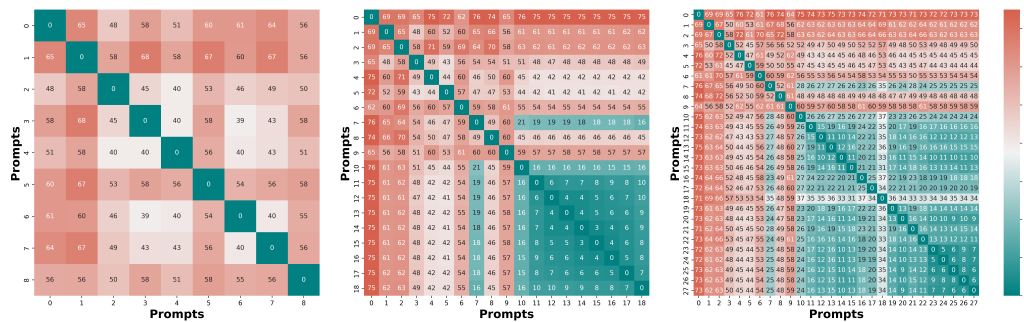
Figure 5: The heatmap visualization presents the angular coverage across all learned prompts through the 2nd, the 3rd, and the 4th round of training. The maximum angular coverage (MAC) monotonically increases from 67.7° in the 2nd round to 75.95° in the final round. The gradual reduction in rate of change in angular coverage towards the final round suggests that the model nearing convergence.
