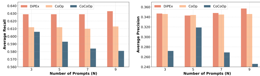
Figure 4: Impact of the prompt length on the MS-COCO dataset. The average recall (AR) and precision (AP) are reported to compare the derived DiPEX against CoOp [24] and CoCoOp [23].
